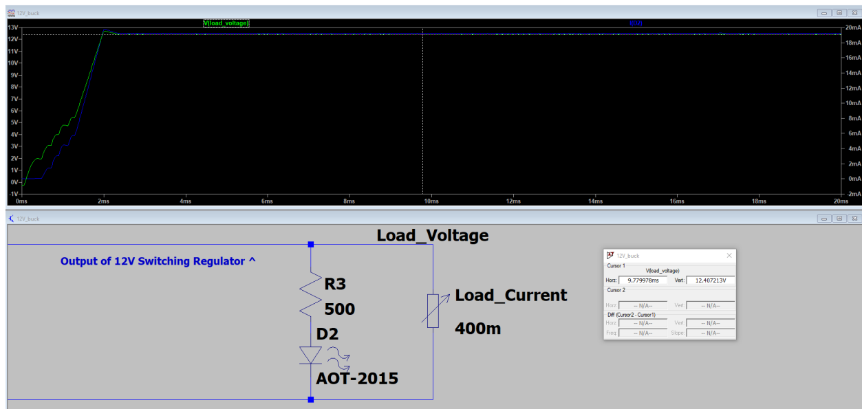
Figure 29; 20mA LED on 12V switching regulator output, transient simulation showing both LED current and output voltage
