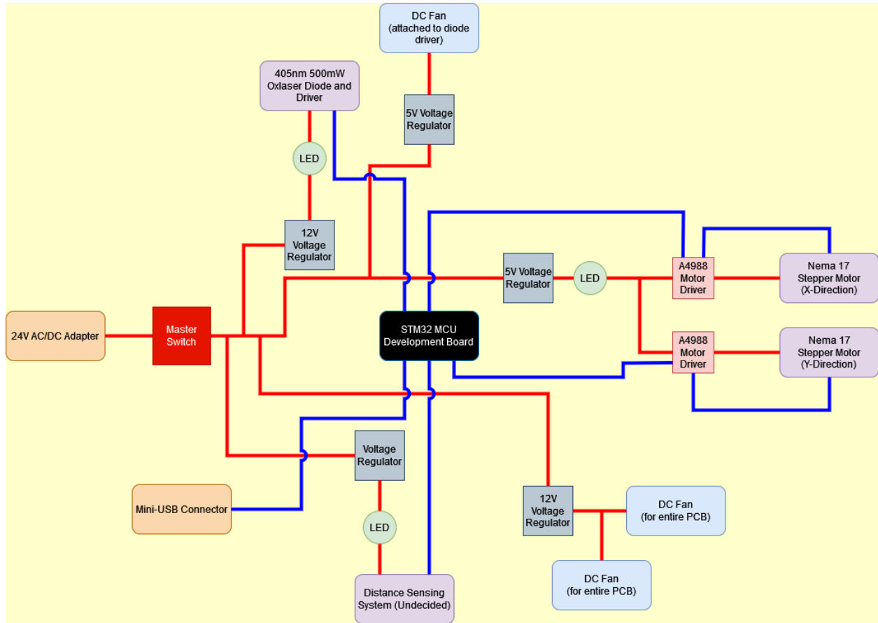
Figure 24; High-Level Design Flowchart
