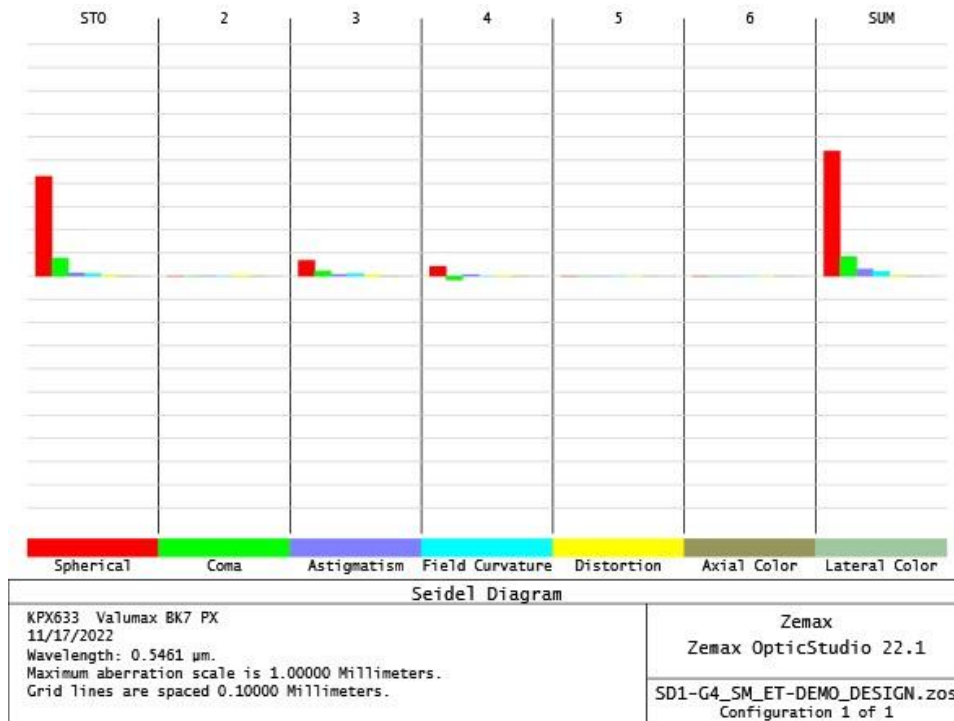
Figure 47; Final Seidel Diagram
