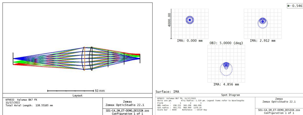
Figure 14, Lens design
