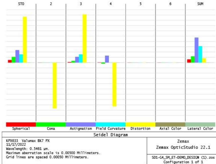
Figure 44; Seidel Diagram for the Second Demo Lens System
