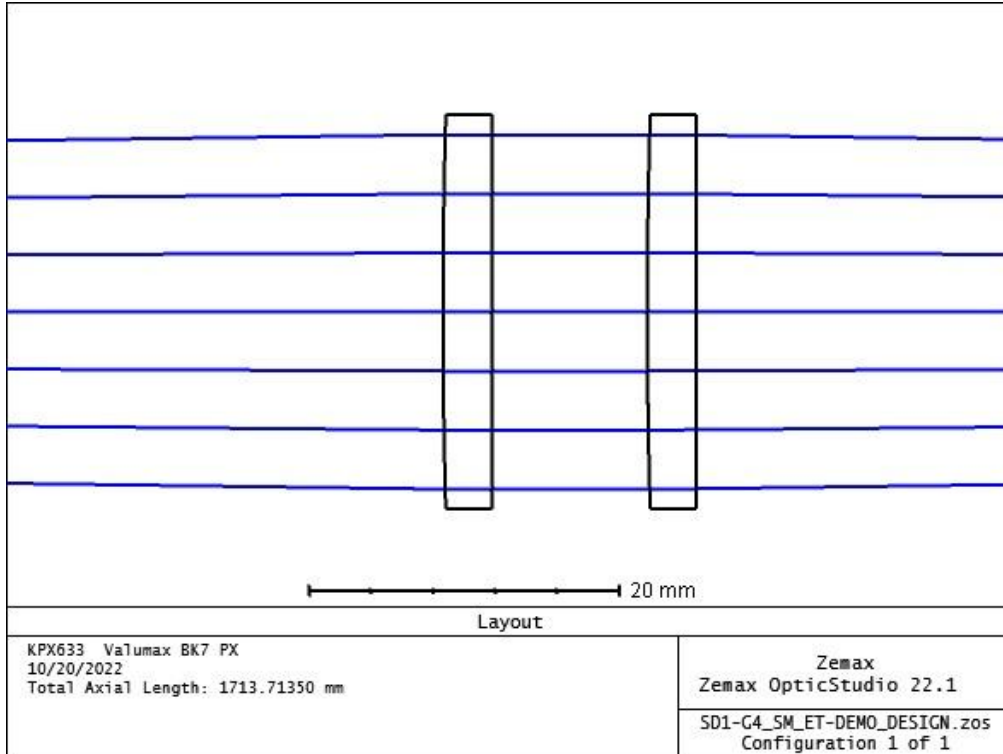
Figure 38; Lens design that Zemax calculated
