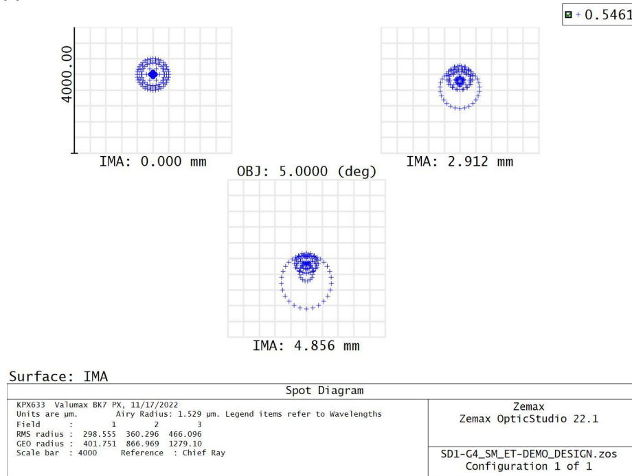
Figure 48; Final Beam Spot Patterns for On and Off-Axis Rays
