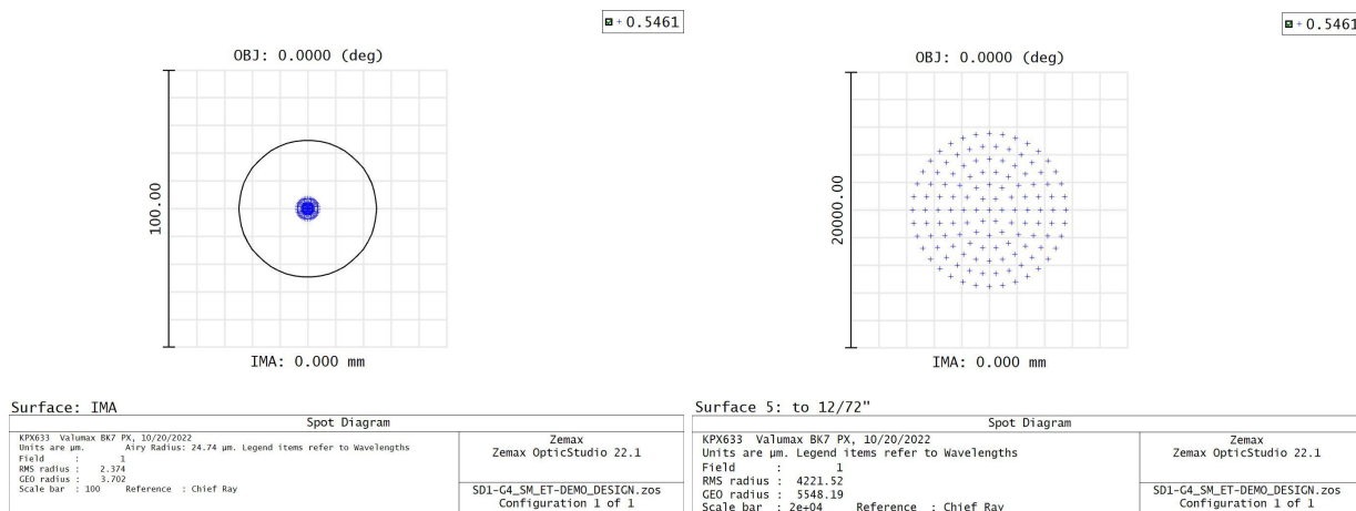
Figure 39; Spot size that Zemax calculated with the an analysis of the results
