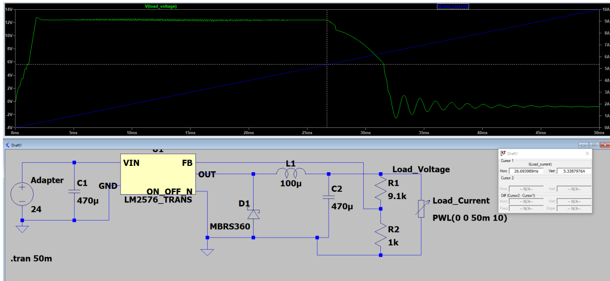
Figure 28; LM2576 Adjustable Switching Regulator schematic and transient simulation, 12V output and 0-10A load range
