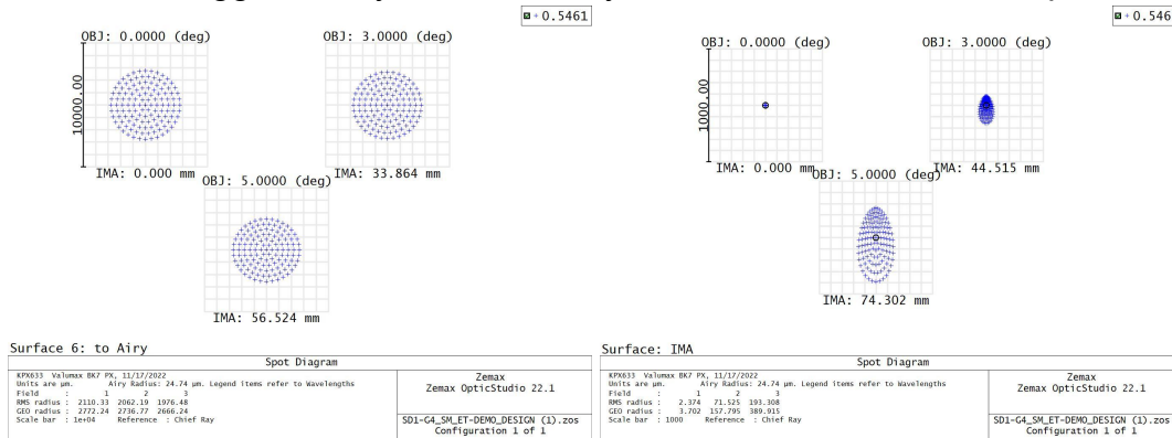
Figure 45; Spot Sizes for Ideal Resolution and Airy for On and Off-Axis Rays
