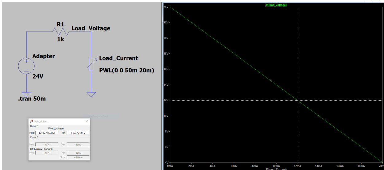
Figure 25; Voltage Divider Regulator schematic and transient simulation, variable voltage output and 0-20mA load range
