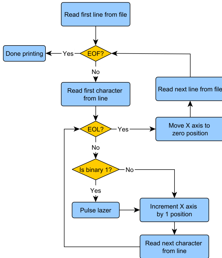
Figure 31; Printing process in MCU firmware
