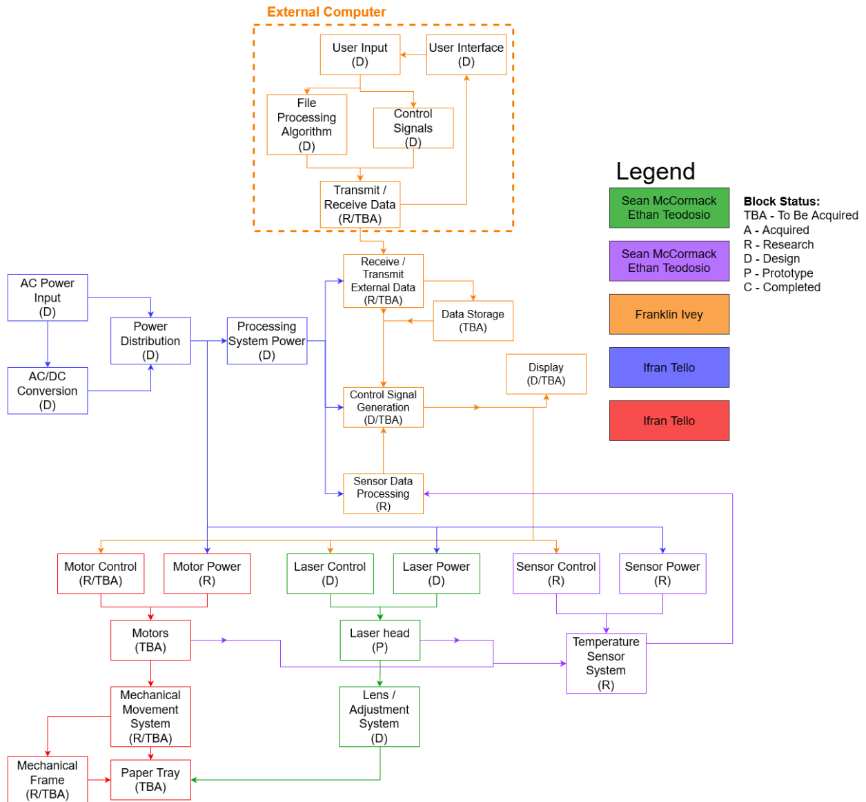
Figure 3; Subsystem block diagram and distribution of work
