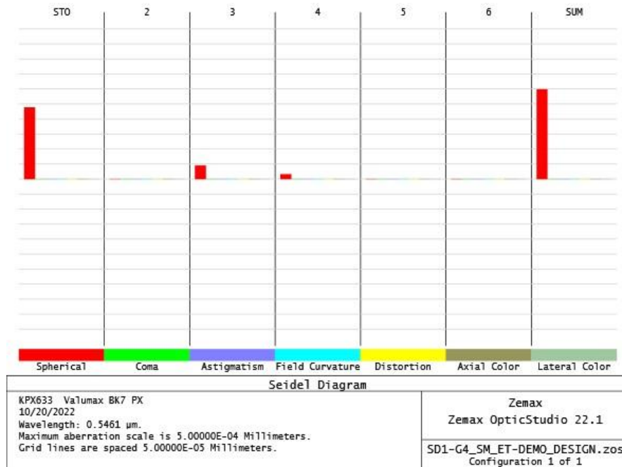
Figure 40; Zemax Seidel Diagram
