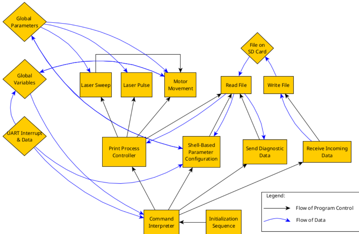
Figure 30; Flowchart of general firmware components and program flow
