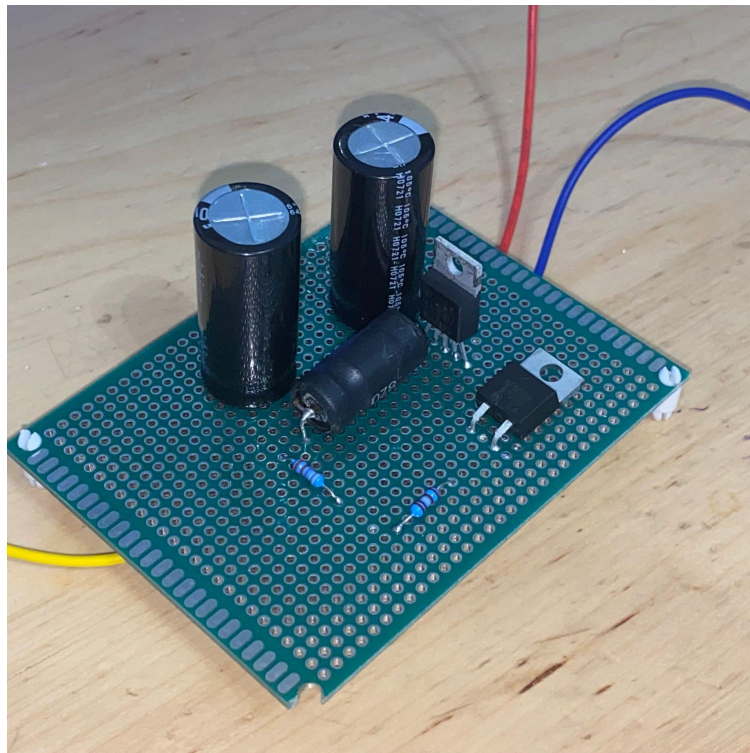
Figure 35; LM2576 Adjustable regulator with 12V output
