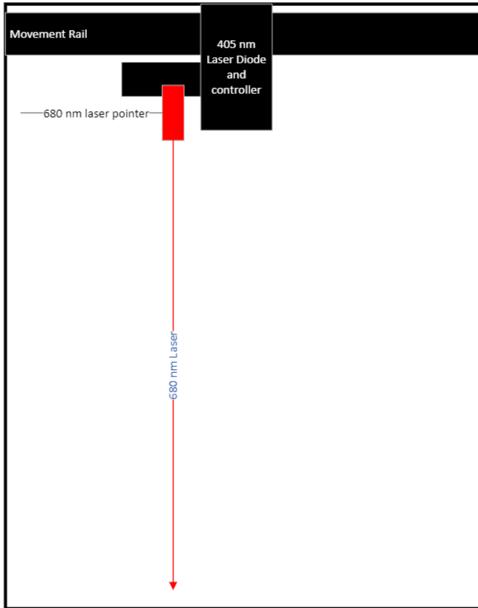
Figure 21, Optical Workspace Detection System mounting option 1
