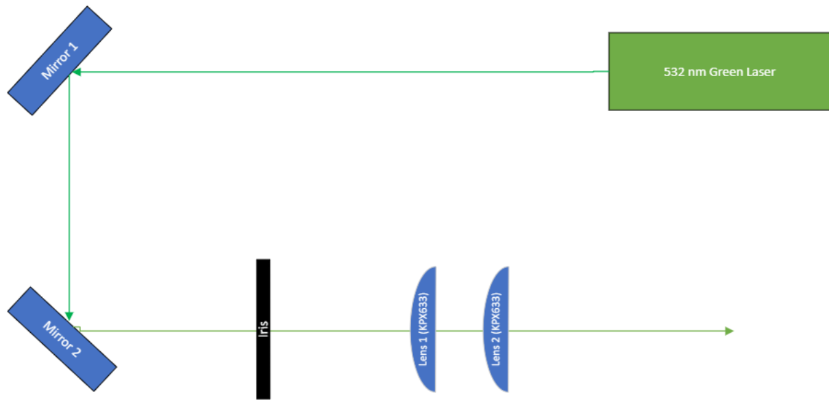
Figure 36; Schematic of the laser setup for the first demo
