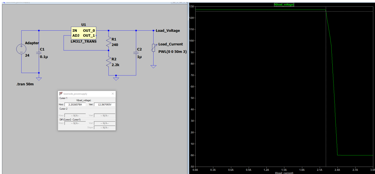
Figure 27; LM317 Adjustable Regulator output schematic and transient simulation, 12V output and 0-3A load range
