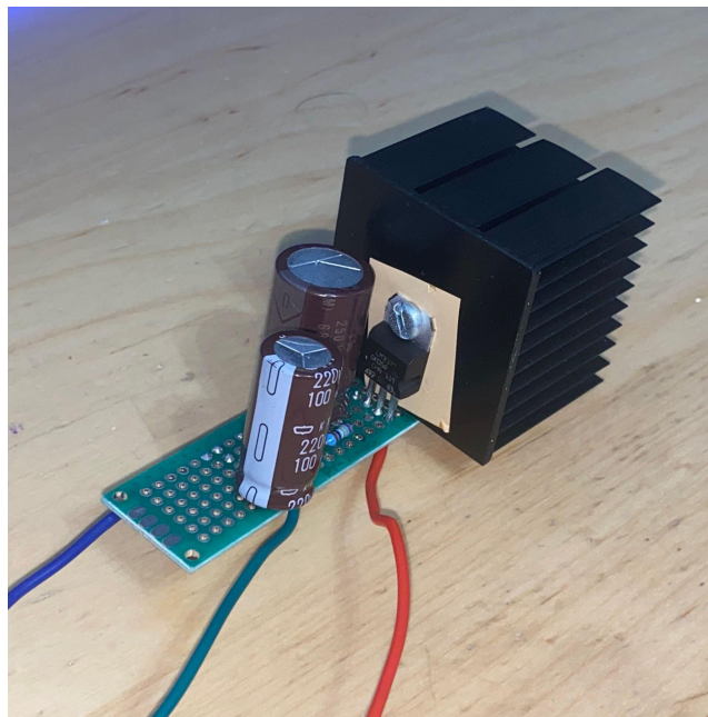
Figure 34; LM317 Adjustable Regulator prototype with 12V output
