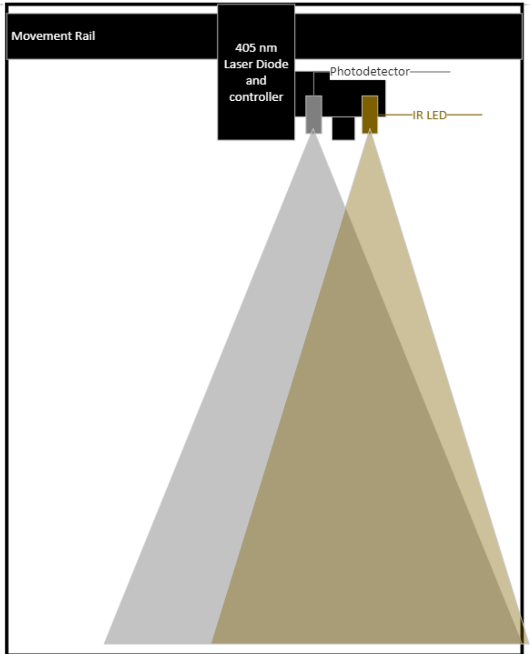
Figure 20; Diagram of how the time of flight method would work
