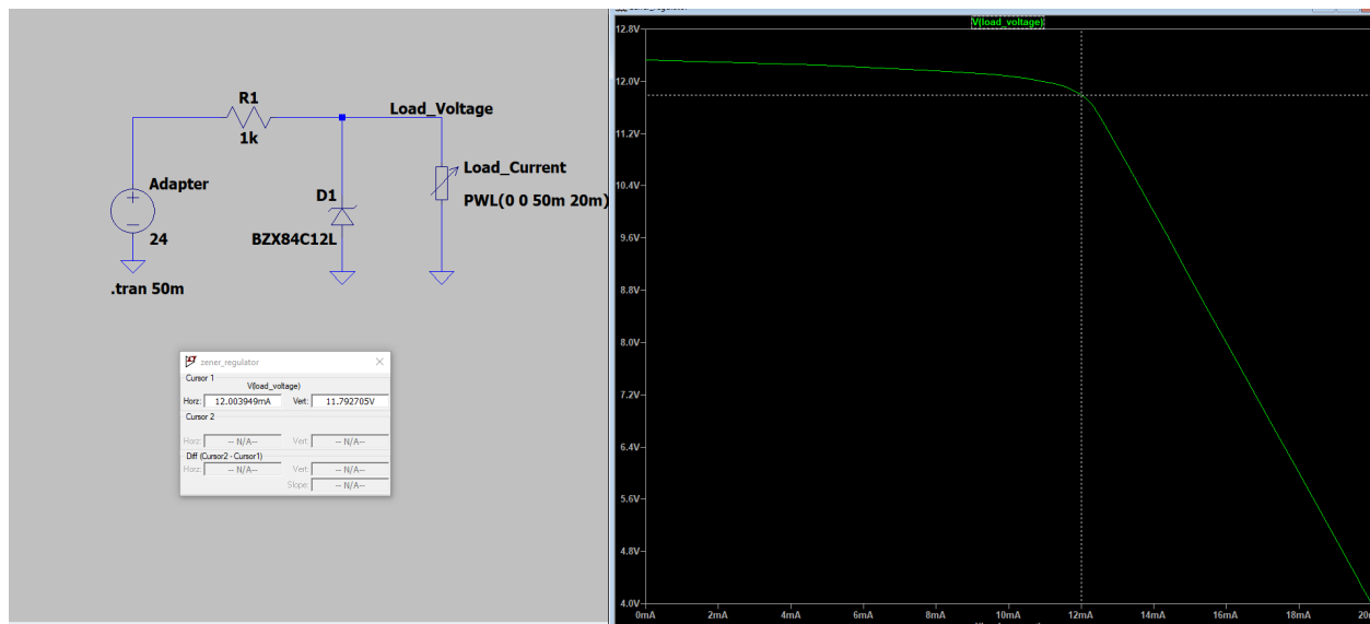
Figure 26; Zener Regulator schematic and transient simulation, 12V output and 0-20mA load range
