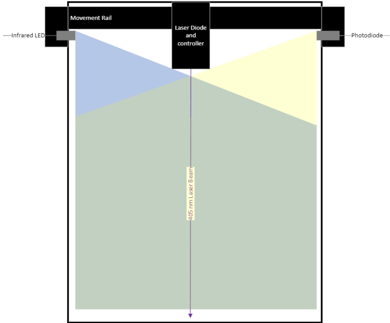
Figure 19; Schematic of how a fire safety system could be designed for our system
